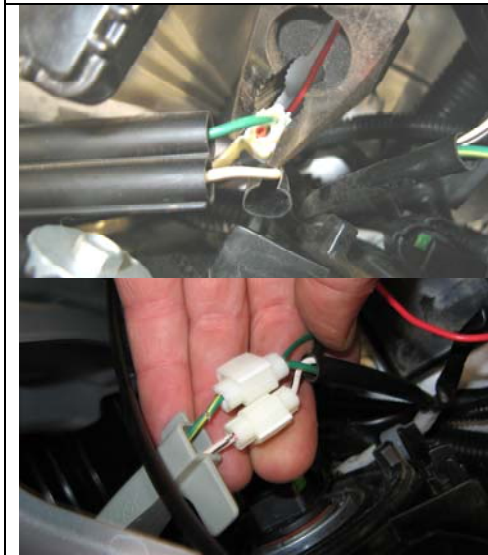
Indicator lamp wiring
