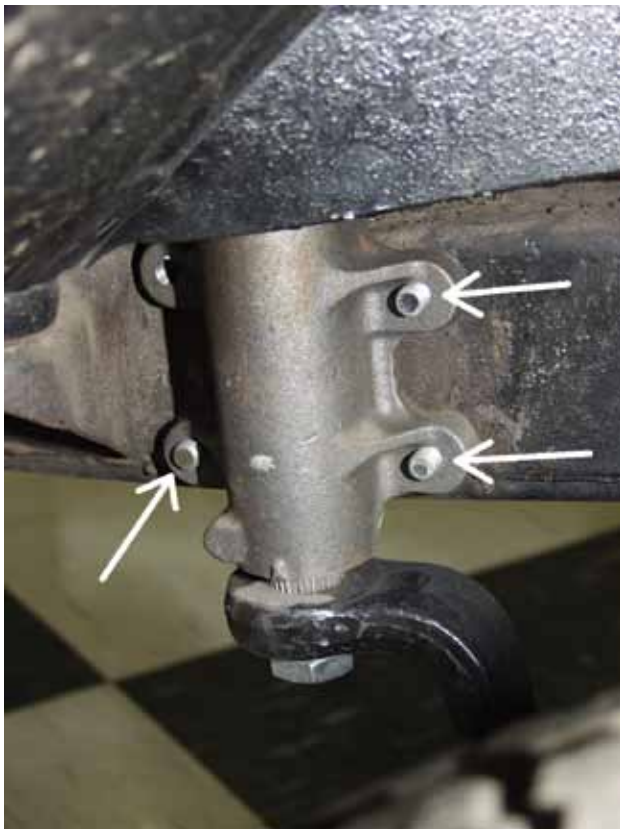
This photo shows the three holes used to mount the box to the frame.
